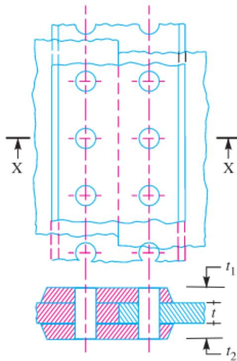
Single riveted double strap butt joint.
