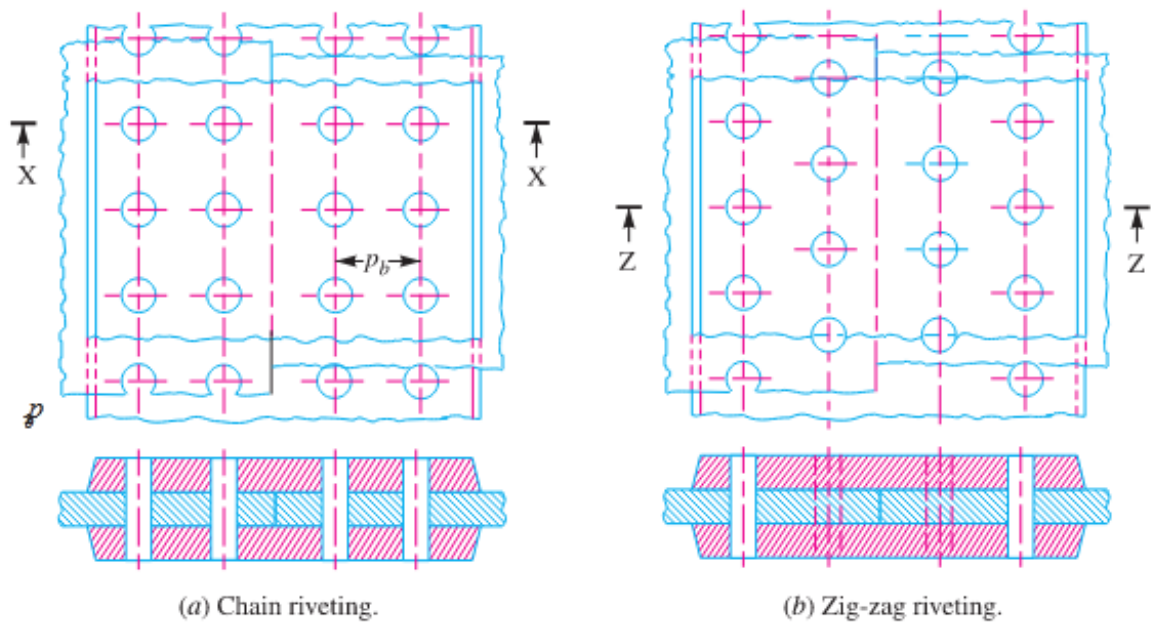
Double riveted double strap (equal) butt joints.
